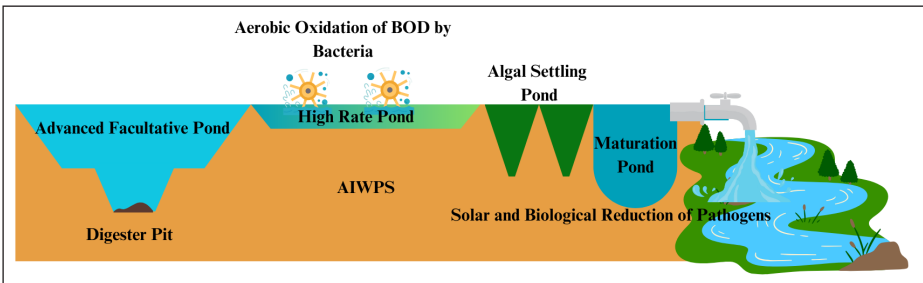
Figure 2: Advanced integrated wastewater pond systems
